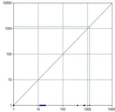
Figure 1: Time taken to solve 64 quantified integer linear arithmetic benchmarks from [19]. The method described in [19] is on the x -axis, our new method is on the y -axis. All benchmarks are solved almost instantaneously by QSAT with the longest run time being 0.08 seconds. This contrasts with 10 timeouts for QT.
