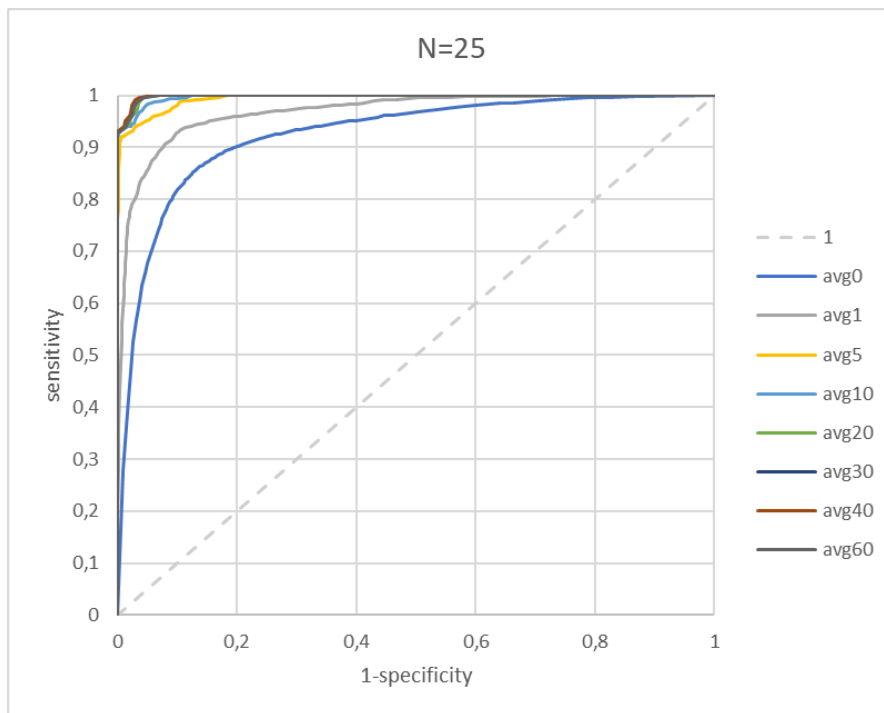
Figure 5. Dependence of sensitivity-specificity on the basic study for different periods (in seconds) of DIC averaging.
