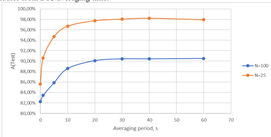
Figure 7. Dependences of COVID-19 diagnosis accuracy (A, Test) from DIC averaging period for preliminary (N=100) and basic (N=25) studies.
