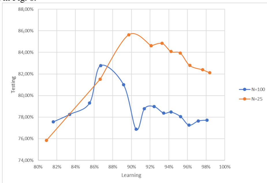
Figure 6. DIC accuracy (Testing) dependence from the discrimination accuracy of learning database (Learning). Data for micromotion analysis settings during the preliminary (N=100) and basic (N=25) studies without DIC averaging.
