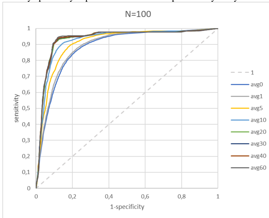
Figure 3. ROC dependence of sensitivity-specificity on the preliminary study for different periods (in seconds) of DIC averaging.
