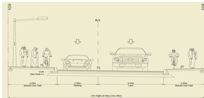
Figure 1: Typical cross-section of the local road (Qatar Highway Design Manual, 2021, vol. 1)
